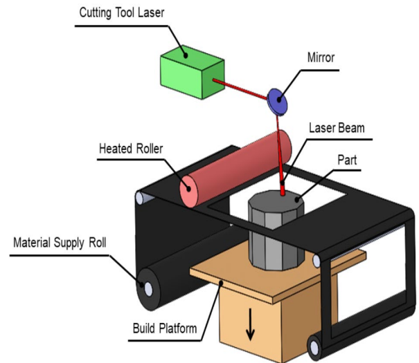
Fig. 7 Laminated Object Manufacturing (LOM) [2]
