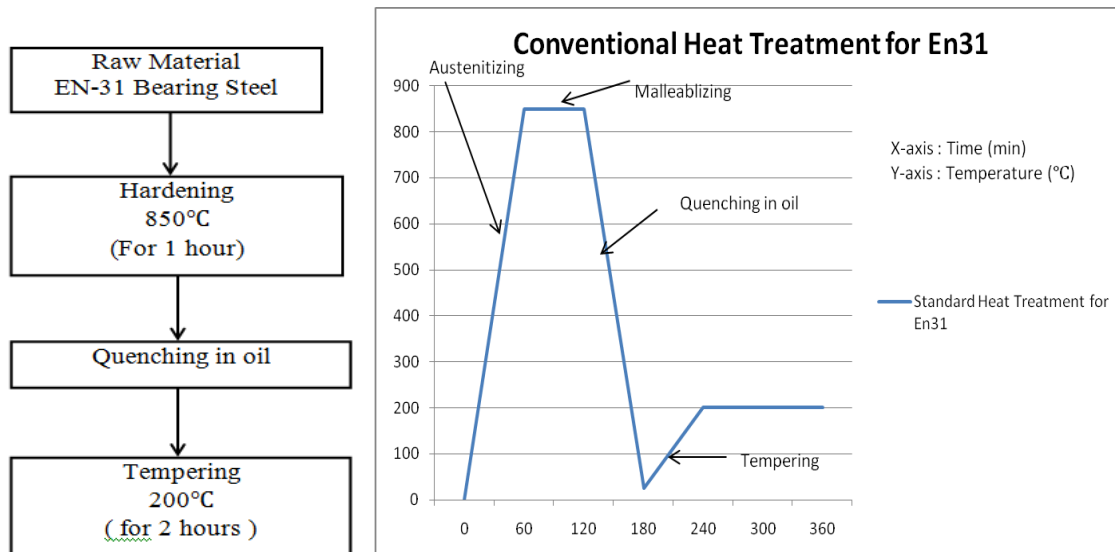
Fig. 1 Process chart for Conventional Heat Treatment
