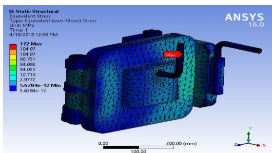
Fig. 8 Equivalent stress distribution of front door
